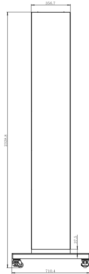
[ FRONT ]
